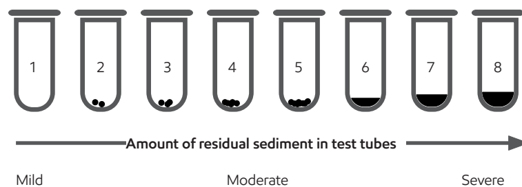
Figure 3: Ultracentrifuge visual sedimentation rating scale
