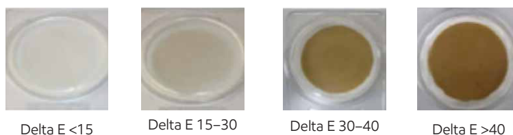
Figure 3: Ultracentrifuge visual sedimentation rating scale
