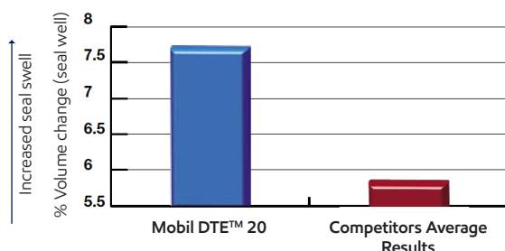
ISO VG 46 Hydraulic Oil in seal swell test NBR-1, 100°C, 168 hrs (run under DIN conditions)
