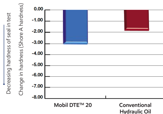
Seal Compatibility 168 hrs, 100°C, NBR -1, Shore A Hardness Run under DIN conditions
