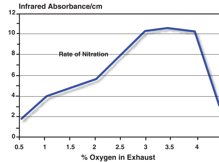
Chart 1. Effects of air/fuel ratio on nitration.
